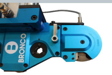
Quick-change cap tip magazine
